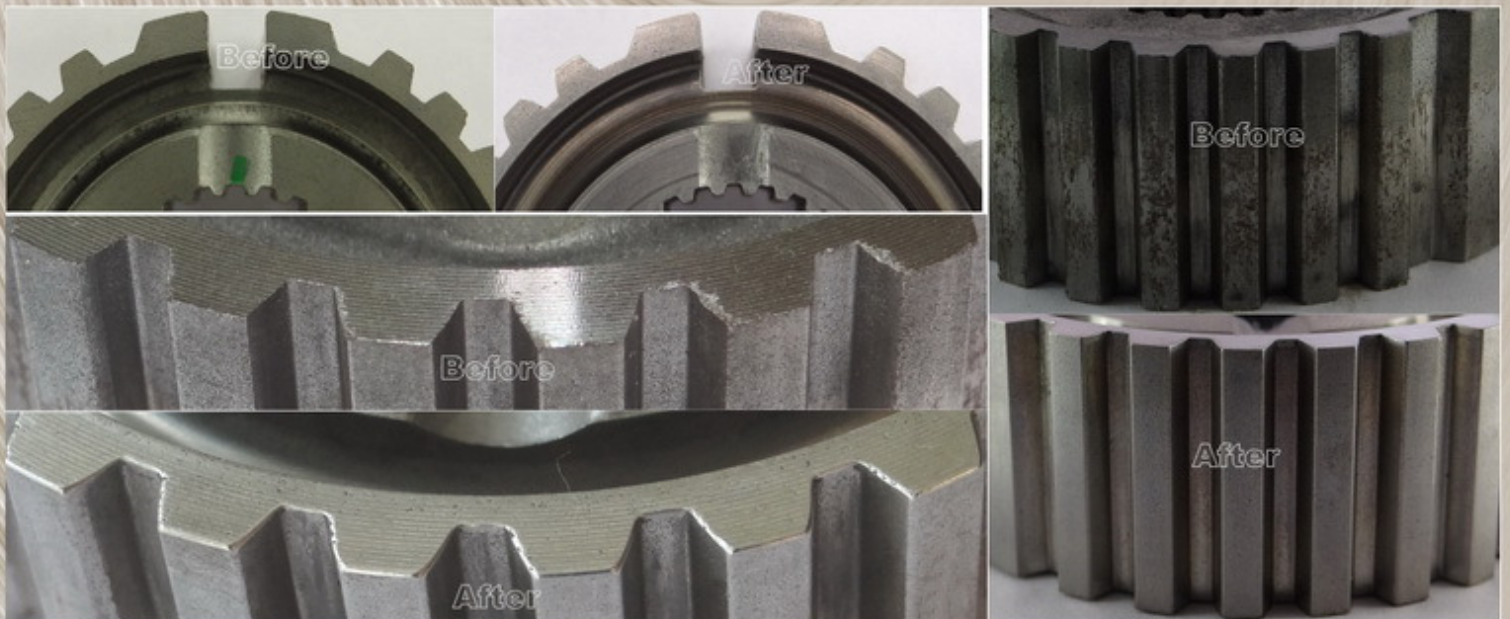
One setting - using IMEXSU Brushes - showing after photo where burr on slot removed, Sharp Edge rediused, Rust removed & Turning marks smoother.
